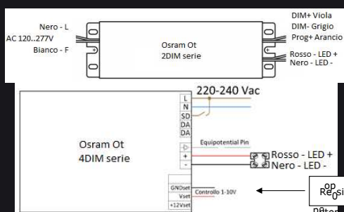
Alimentazione by Osram OT series 2DIM e 4DIM
